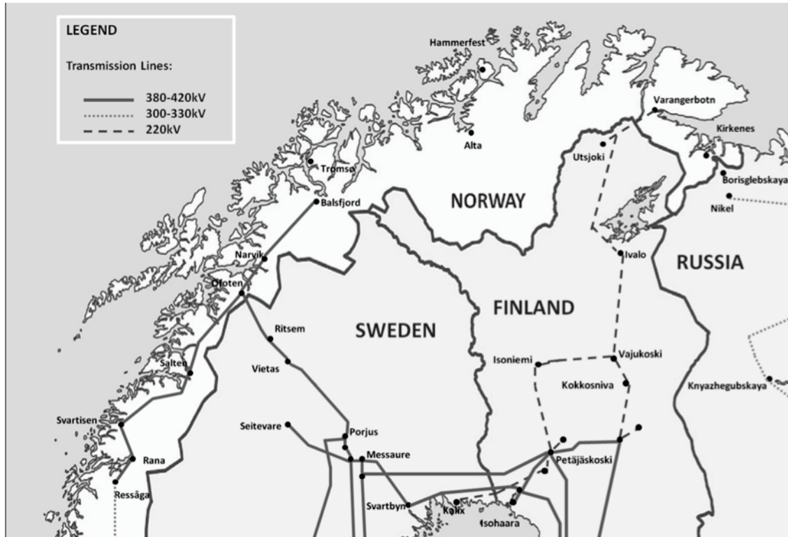
Fig.1: Transmission Lines between 220kV and 420kV in Northern Scandinavia
