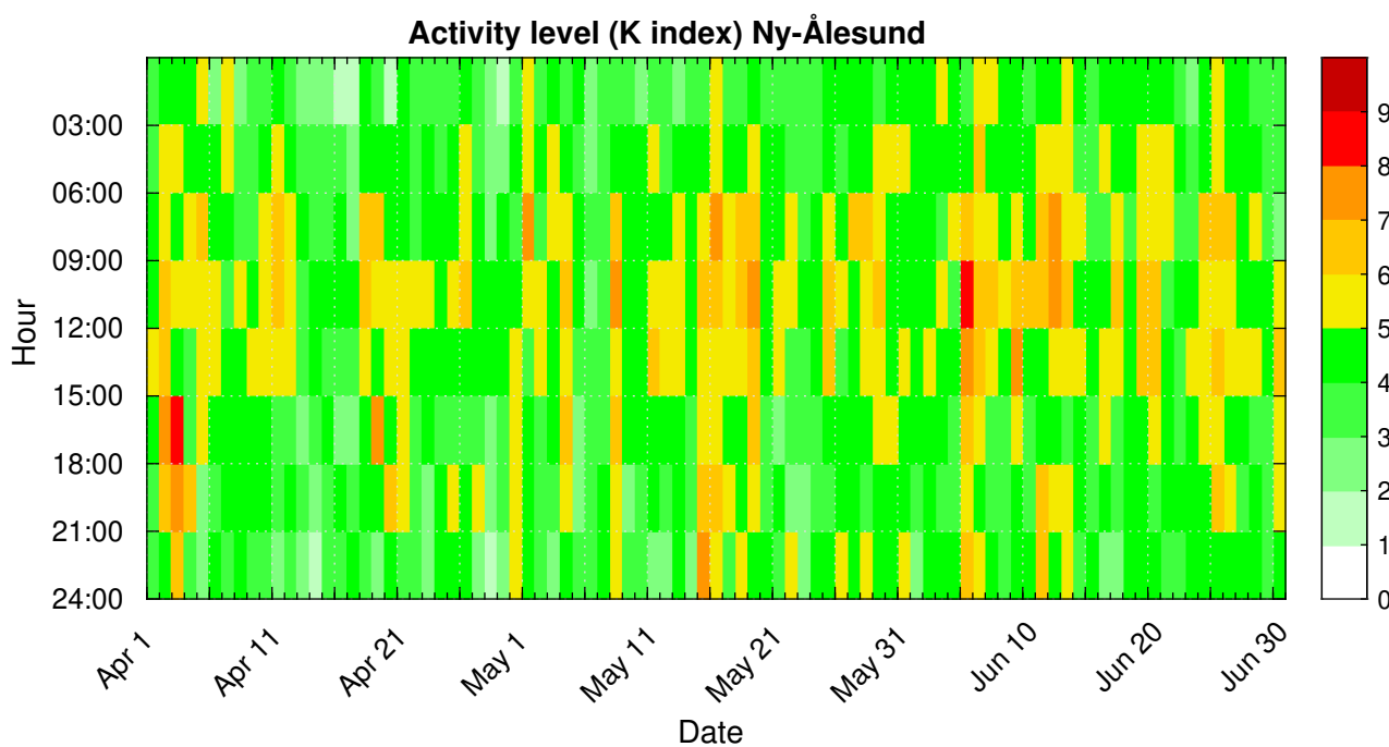
Figure 6: K index at Ny-Ålesund.
