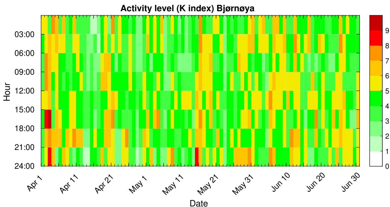
Figure 7: K index at Bjørnøya.
