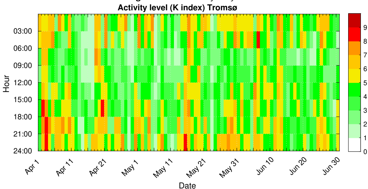
Figure 8: K index at Tromsø.
